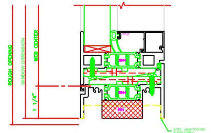
241 SILL 325 CASEMENT OUT BUTT HINGES
